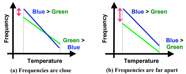
Figure 3: The relationship between the ring oscillator frequency distance and the probability of a PUF output flip.
