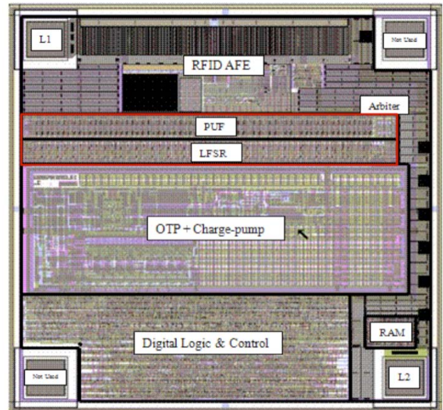
Figure 3. The floorplan of a PUF-enabled RFID.
