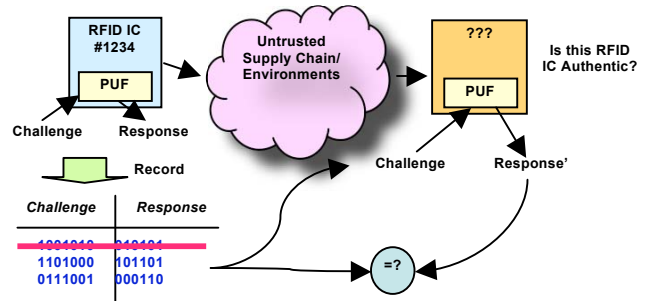
Figure 2. The overview of the PUF-based RFID authentication procedure.
